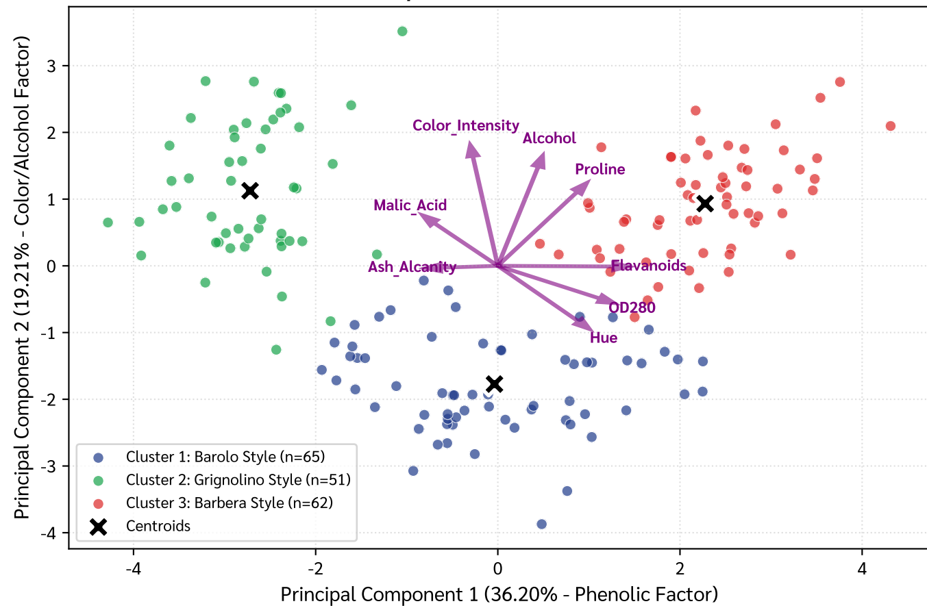
(a) 2D PCA Biplot & K-Means Clusters ( K = 3 )
